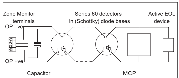
Fig.3 Zone connection – diode bases with active EOL device
